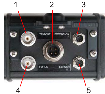
Pedal Force Display - rear panel
